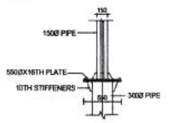
DETAIL A FOR PIPE JOINT
